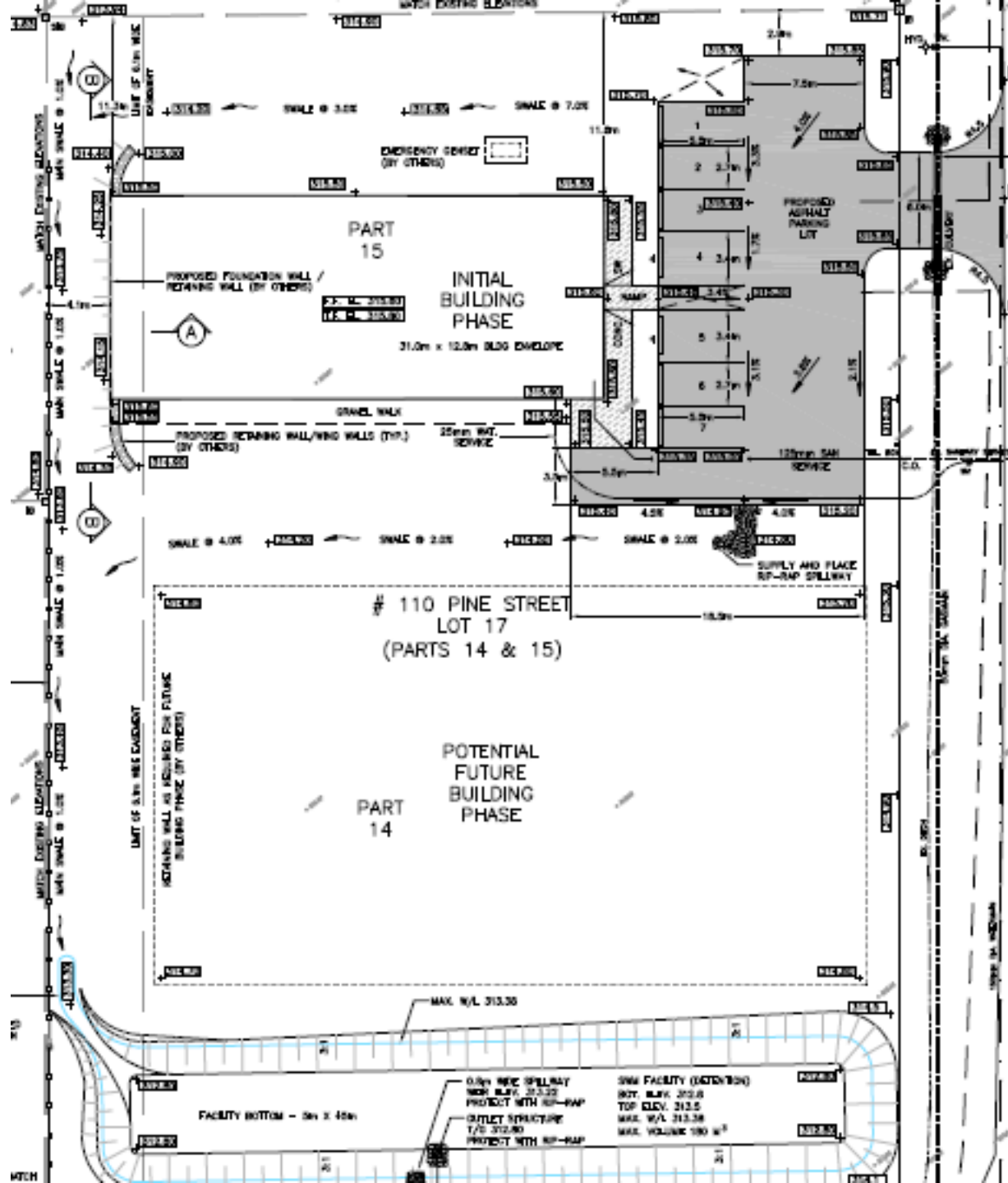
Natural Pharm Industry Inc. Site Grading and Drainage Plan
